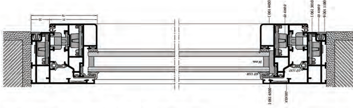
SEC B-B
